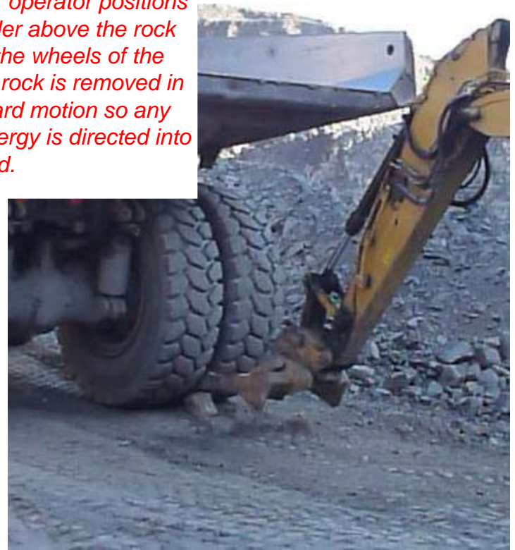
'Prodder' attaches to backactor using quick hitch coupler
